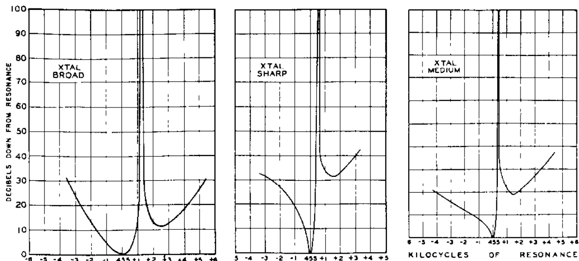
Figure 15. Crystal Curves
