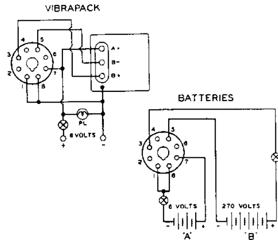
Figure 10. Octal plug wiring diagram
