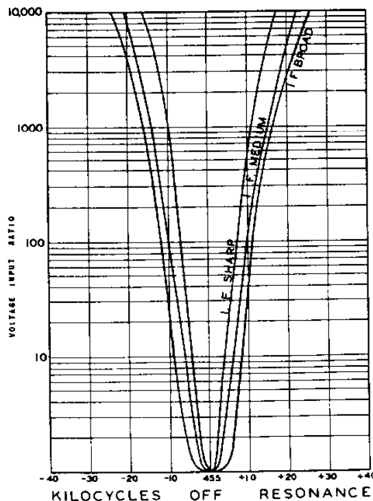
Figure 14. Selectivity Curves
